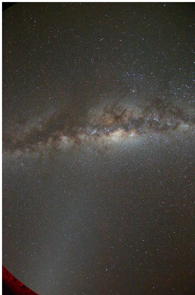
Figure 3 — Zodiacal light
