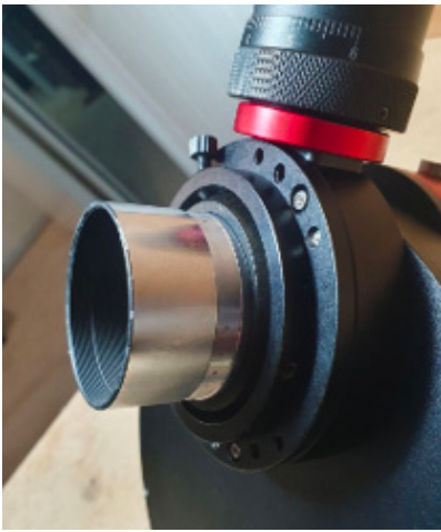
Figure 6 — Camera adapter coupling where a loose screw caused micro-vibrations and uncorrectable guiding drift.
