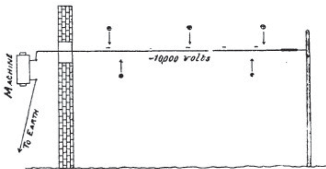
Figure 1 — Earth
