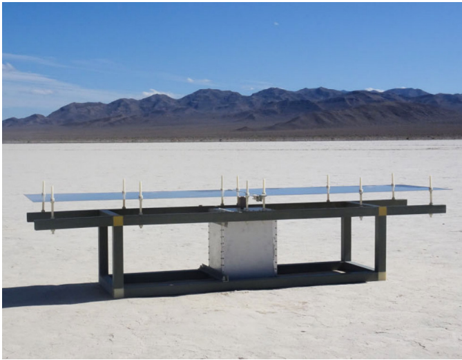
Figure 2 — A Mapper of the IGM Temperature experiment instrument at the testing site in Nevada, USA. Credit: MIST team/Monsalve et al. (2024).
