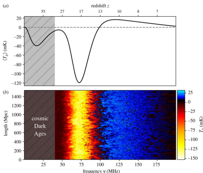
Figure 1 — A simulation of the HI signal across time and frequency. This model shows a changing signal over the different eras of the early Universe: the Dark Ages, Cosmic Dawn, and Epoch of Reionization. Credit: Fialkov et al. (2024)
