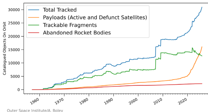
Figure 1 — The number of objects in orbit over time. This includes active and defunct satellites (orange line), trackable fragments (debris larger than approximately 10cm; green line), abandoned rocket bodies (red line), and the sum total of those three components (blue line). Figure credit: Aaron Boley/Outer Space Institute.
