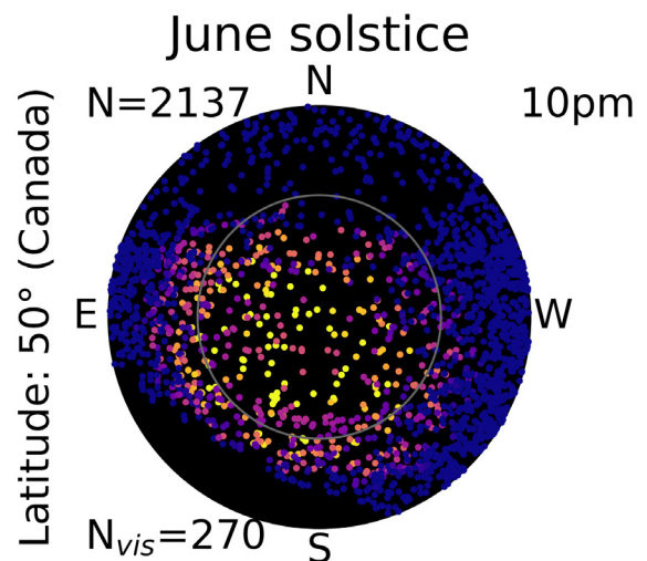
Figure 2 — An all-sky plot showing the positions and brightnesses of 65,000 planned megaconstellation satellites at 10 p.m. on the summer solstice from 50° north latitude. N is the number of sunlit satellites above the horizon, and N_{vis} is the number of naked-eye visible satellites; yellow shows the brightest satellites and blue shows the faintest. Figure based on Lawler et al. (2022).
