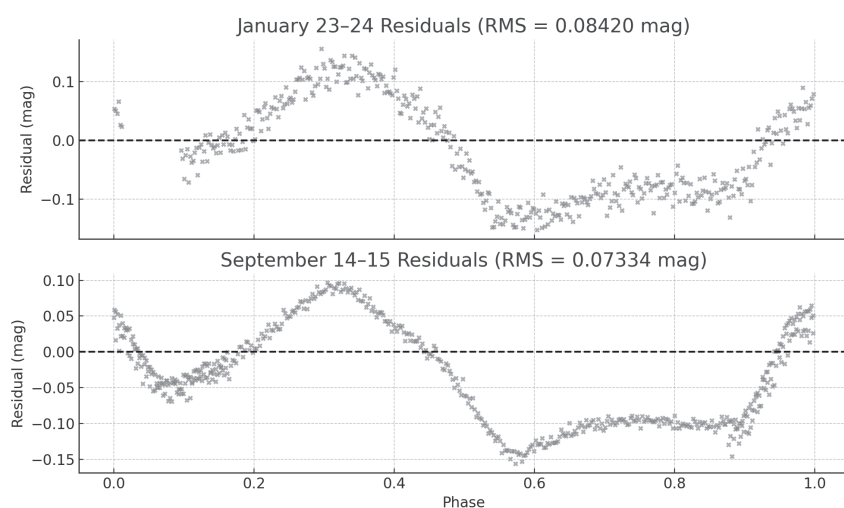
Figure 5 — Residuals between observed and modelled flux. (a) January 2023 data shows modest scatter and wave-like structure. (b) September 2023 data exhibits reduced RMS and symmetrical distribution, indicating a more precise fit.
