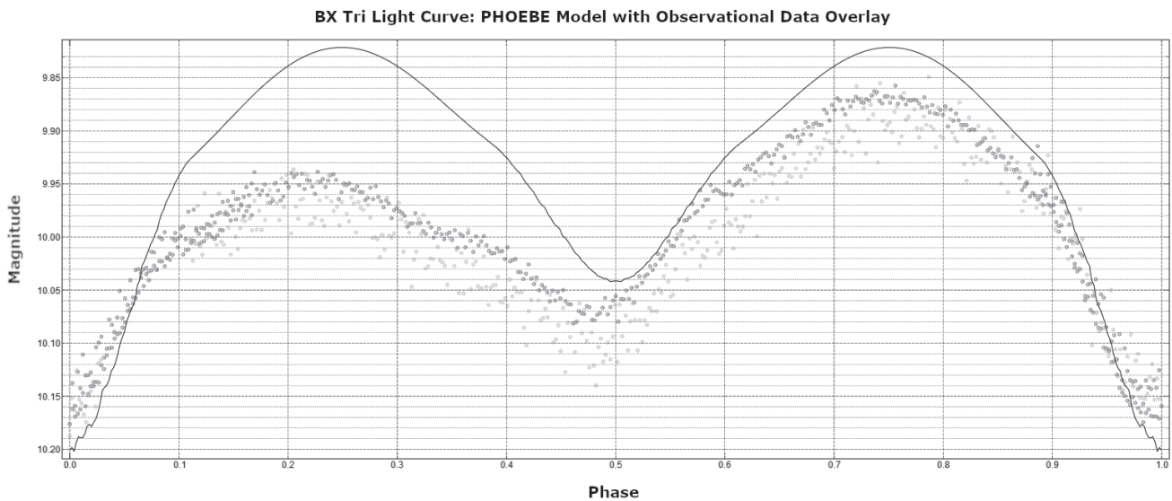
Figure 4 — Comparison between the PHOEBE-simulated light curve (solid line) and observed photometric data (gray points) for BX Tri. The model captures the overall shape of the light curve, including eclipse depths and timing, though it does not reproduce the observed asymmetry in the maxima (O’Connell effect).
