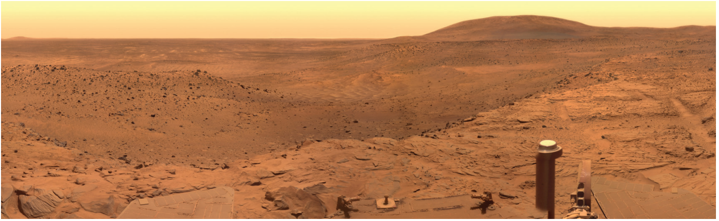
Figure 1 — A panorama of Mars's West Valley captured by the Spirit rover. Features in this image: Tsiolkovski Ridge (hill on the left), Grissom Hill (behind Tsiolkovski Ridge, on the horizon, about 8 kilometres away), and Husband Hill (above Spirit's mast, 800 metres away). Image credit: NASA/JPL/Cornell/James Convin.
