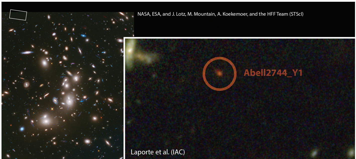
Figure 4 — A deep image of the cluster Abell 2744 acquired by the Hubble Space Telescope (left) and an enlargement of the distant galaxy Abell2744_Y1 (right). Credit: NASA, ESA, and J. Lotz, M. Mountain, A. Koekemoer, and the HFF Team (STScI) Nicolas Laporte et al. (IAC)
