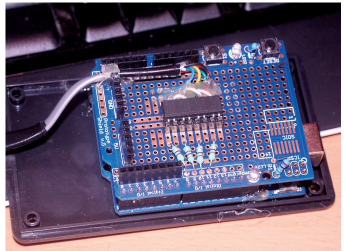
Figure 4 — The top of the prototype shield after wiring.
