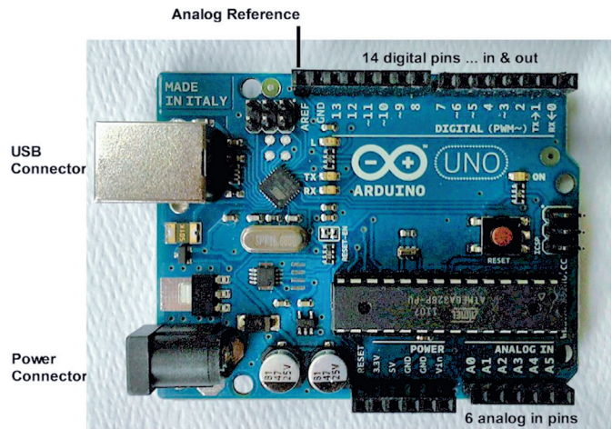
Figure 1 — The Arduino Uno with connections identified.
