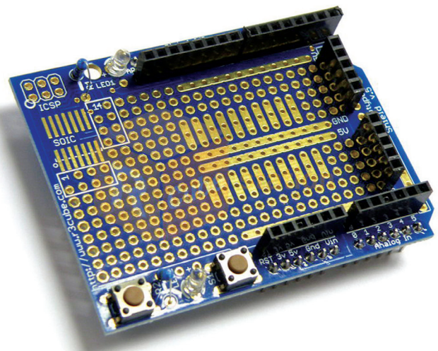
Figure 2 — The front of the Arduino prototype shield.
